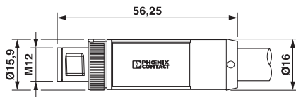
Dimensional drawing
